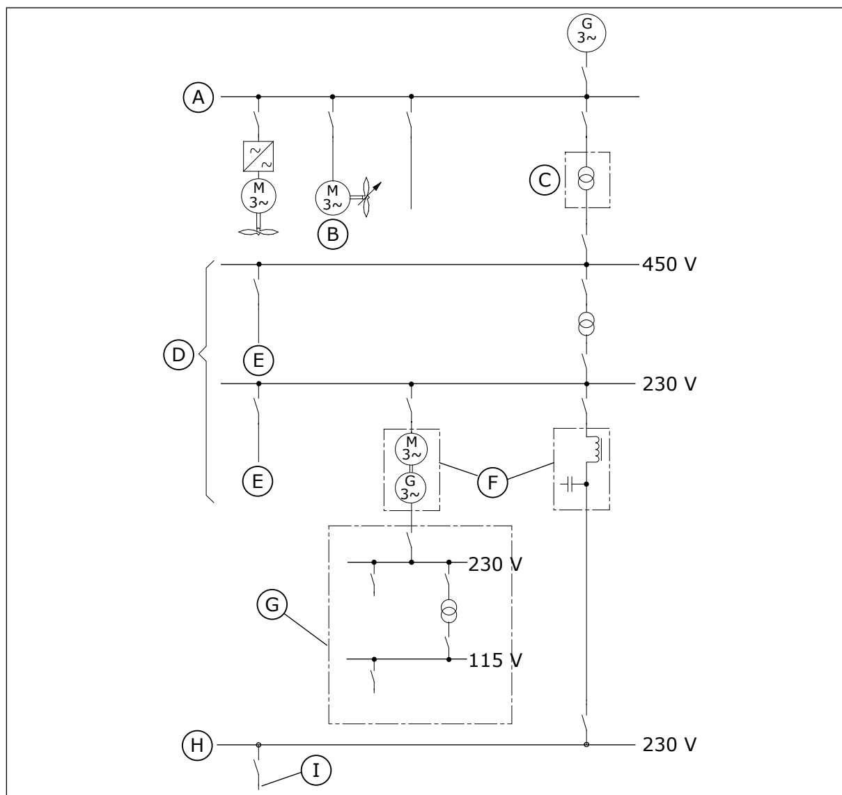
Fig. 12: The installation zones in a marine environment
