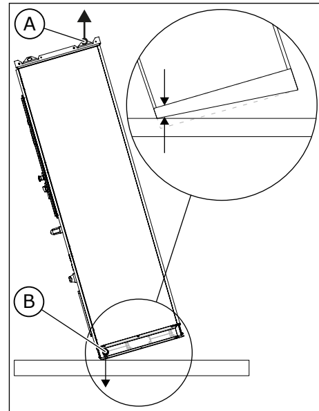
A. The lifting hole B. The springs at the bottom
